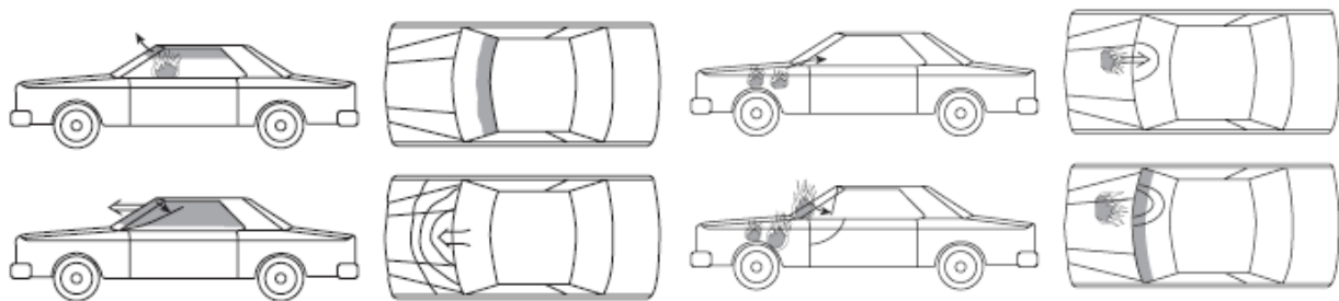
FIGURE 25.8.1.1(b) Fire Pattern Development from an Engine Compartment Origin.
