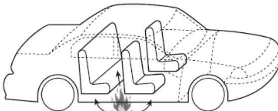
FIGURE 11.4.1.1 Pool Fire Burning Under Vehicle.
